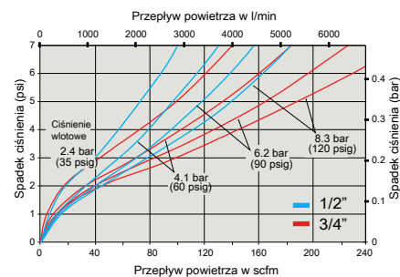
Smarownica 1/2" & 3/4"
