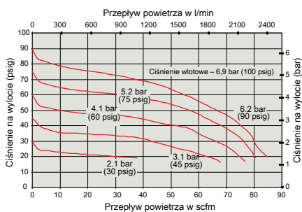
Regulator 1/4"
