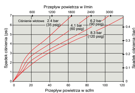
Smarownica 3/8"
