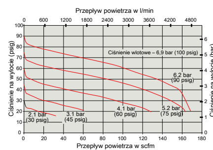
Regulator 3/8"
