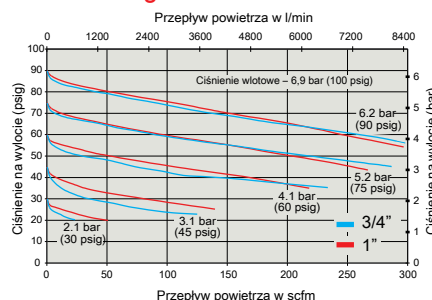
Regulator 3/4" & 1"
