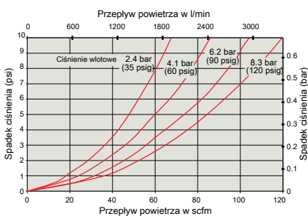
Filtr 3/8"
