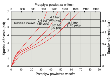
Smarownica 1/4"
