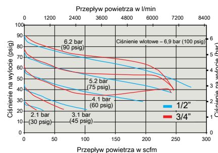
Regulator 1/2" & 3/4"
