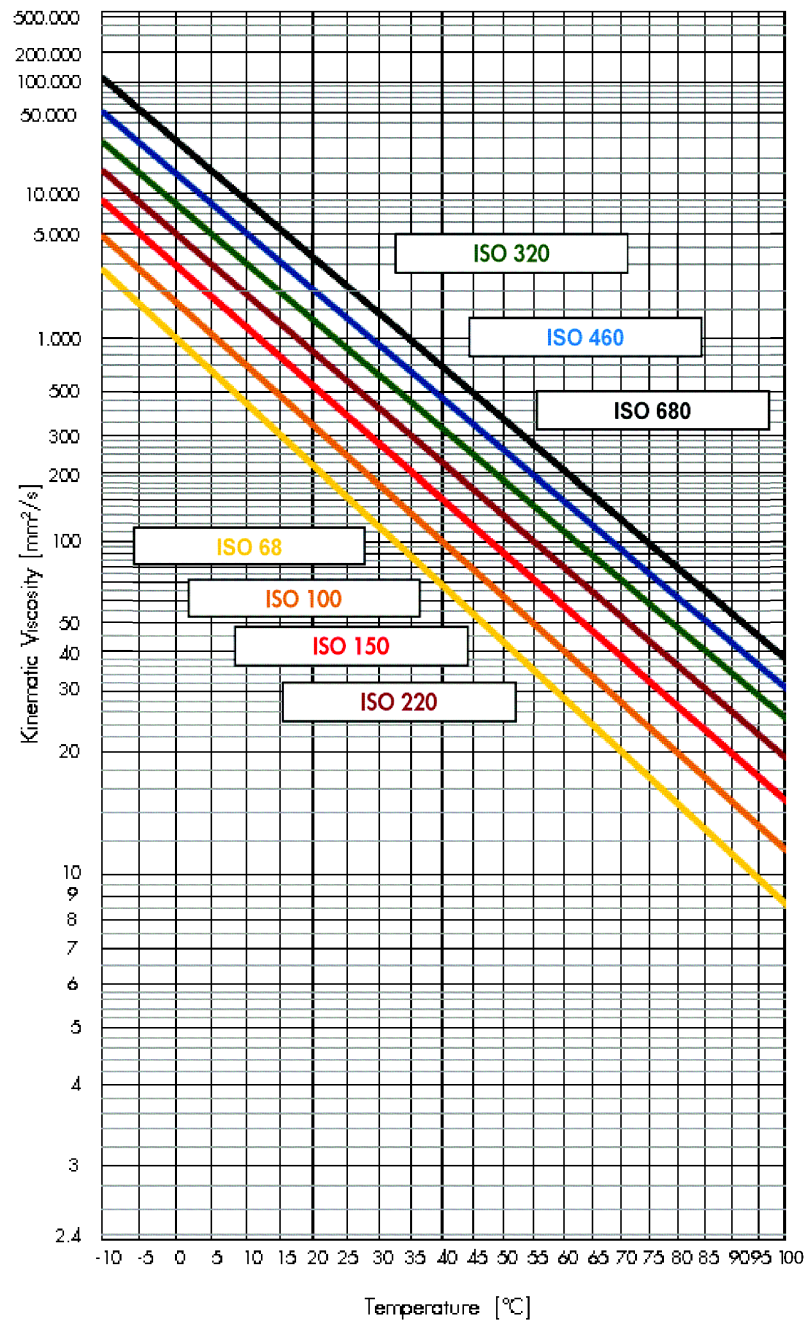
Viscosity - Temperature - Diagram
